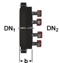
Flange with boreholes according to DIN EN 1092 part 2
